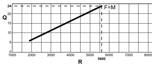
Abb.52 Last Tzerra Ace 24DS
