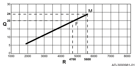
Abb.53 Last Tzerra Ace 28C
