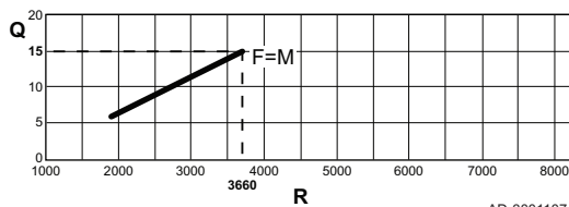
Abb.51 Last Tzerra Ace 15DS
