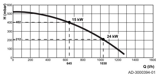
Abb.79 Tzerra Ace 15DS - 24DS
