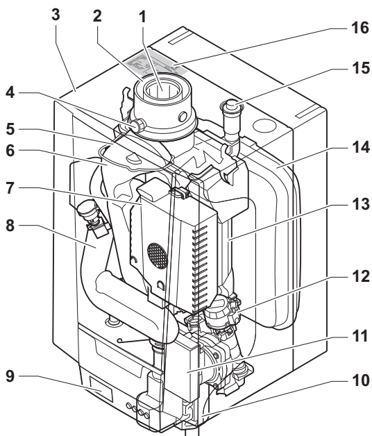
Abb.1 Tzerra Ace 15DS - 24DS
